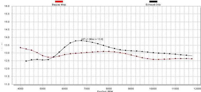
Lambda and Temps vs. RPM Bazzaz Map, Exhaust Only
