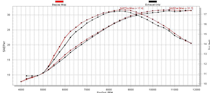
SAE Corrected Wheel Power vs. RPM Bazzaz Map, Exhaust Only
